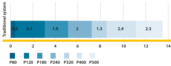
Abrasive consumption – Traditional system: Average 13,3 pcs
